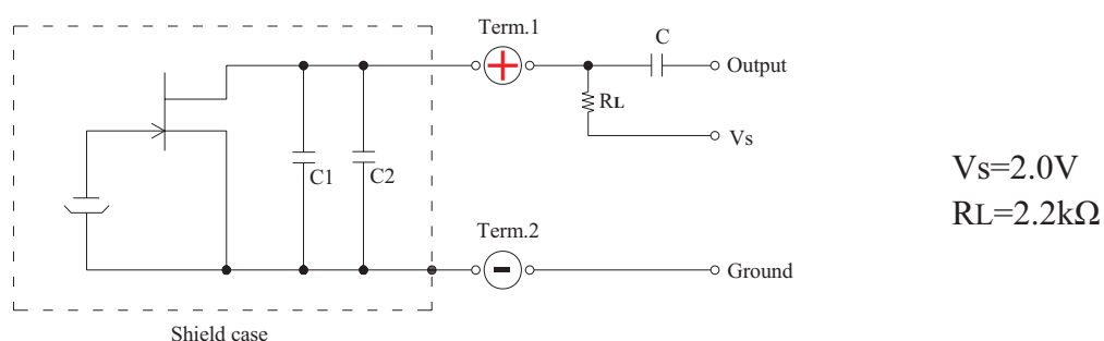
Fig. 5-1 Schematic Diagram
