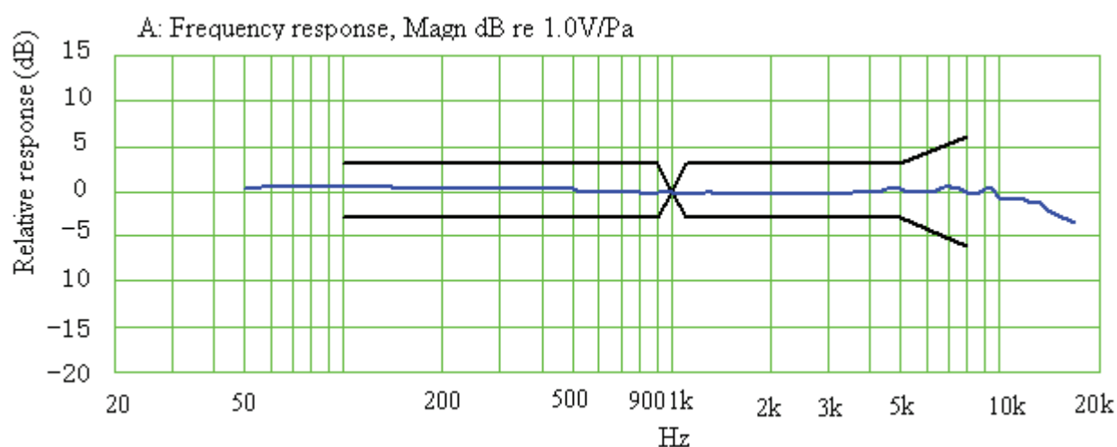
Fig. 4-1 Frequency Response
